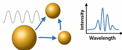
SCATTERING, ABSORPTION, AND EXTINCTION
